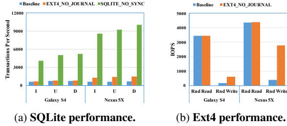
Figure 2: Database and file system performance with optimizations. Figure (a) shows the transaction throughput of single op transaction in SQLite; I: Insert, U: Update, D: Delete. Figure(b) illustrates the 4KB random read / write IOPS of the Ext4 file system.
