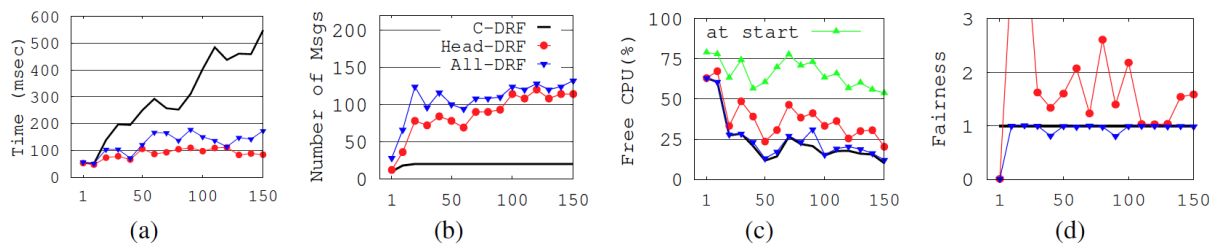
Figure 6: Evaluating C-DRF, Head-DRF, All-DRF. X-axis shows the number of applicants (§ 6.3 for details).
