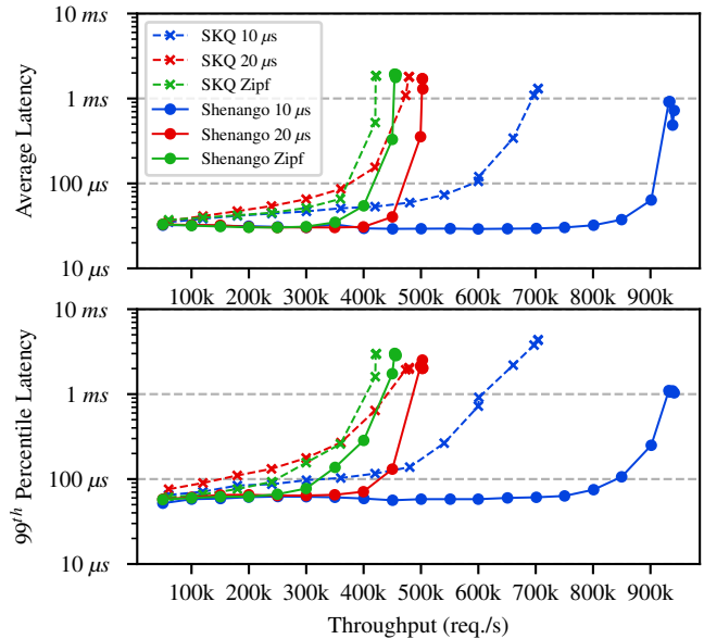
Figure 11: The latency response of three workloads running on Shenango and SKQ. SKQ uses CPU affinity scheduling policy for 10 \mu s, 20 \mu s benchmarks; CPU affinity and best of two with work stealing for the Zipf-like benchmark.
