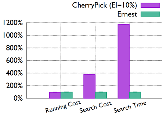
Figure 9: Comparing Ernest to CherryPick (TPC-DS).
