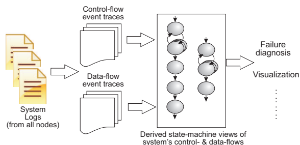
Figure 1: SALSA's approach.
