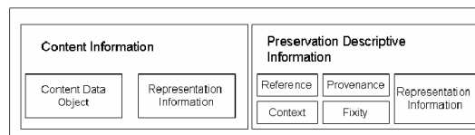
Figure 1 - AIP structure in OAIS [1]
