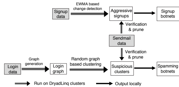
Figure 1: The Architecture of BotGraph.
