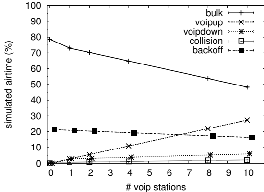
Figure 11: Simulated Softspk airtime usage versus the number of active VoIP streams, in the presence of 802.11b UDP uplink bulk traffic (c.f. Figure 4).
