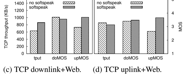
Figure 14: VoIP in combination with bulk TCP traffic (802.11g protected mode, no opt-out). Only five VoIP stations are active. In (c) and (d) the remaining five stations engage in Web traffic. The throughput measured is that of bulk TCP.
