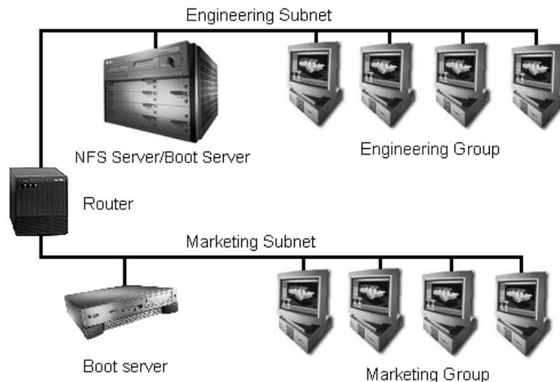
Figure 1: Example JumpStart environment.
