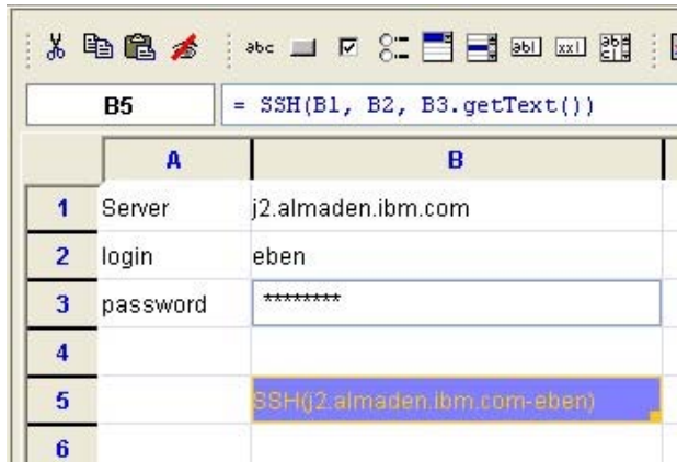
Figure 3: Creating an SSH connection.
