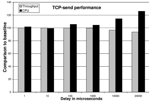
Figure 4: Performance of an e1000 microdriver.
