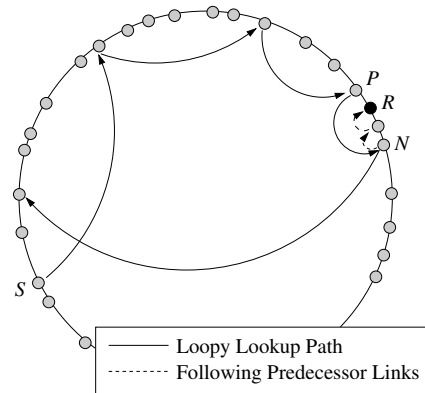
Figure 4: Routing loops . In Chord, if a lookup passes by the correct successor on account of non-transitivity, a routing loop arises. The correctness of lookup can be improved in such cases by traversing predecessor links.
