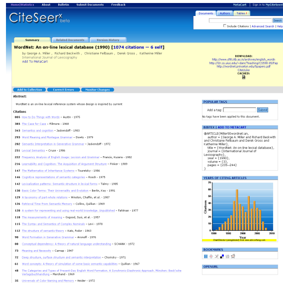
Figure 5: Document Summary
