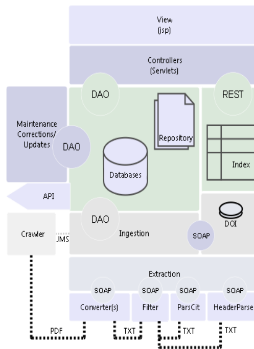
Figure 1: SeerSuite Architecture
