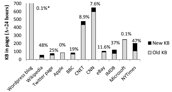
Figure 9: Byte turnover: 24 hours.
