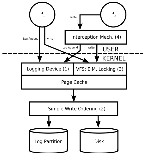
Figure 1: Valor Architecture
