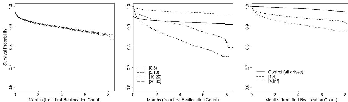
Figure 11: Impact of reallocation count values on survival probability. Left figure shows aggregate survival probability for all drives after first reallocation. Middle figure breaks down survival probability per drive ages in months. Right figure breaks down drives by their number of reallocations.
