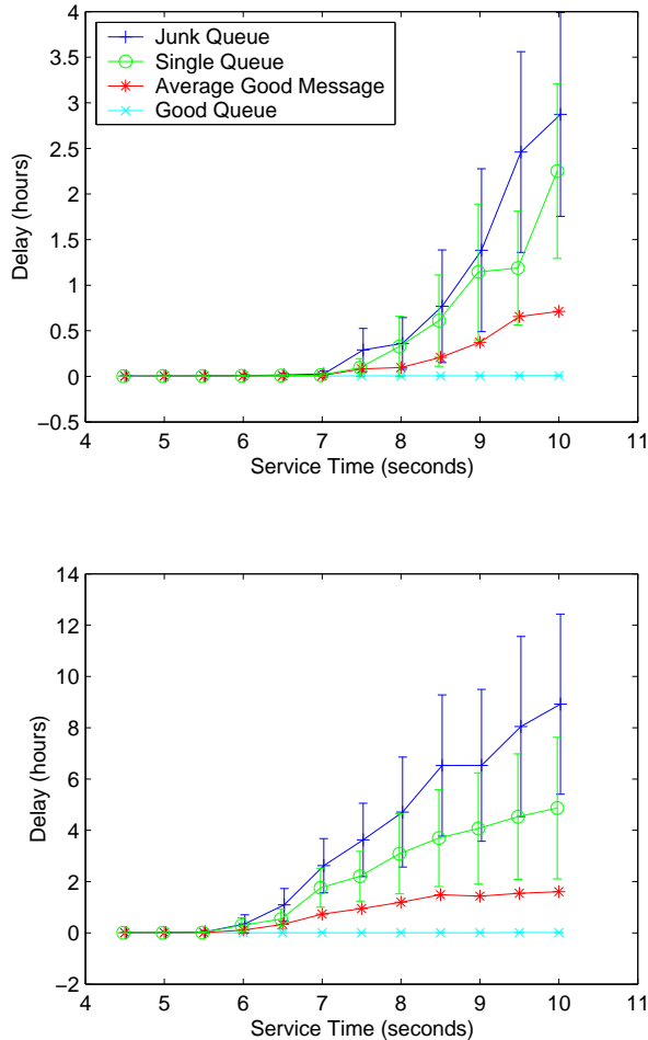
Figure 9: Average delay against server performance ( t_{SCAN} ) for the original model ( \circ ), good queue ( \times ), junk queue ( + ) and average good ( * ). The top plot corresponds to normal and the lower to SoBig traffic loading. With a single queue, a highly rated server is needed to provide good performance under heavy loading, while with prioritization good mail has consistently low delays even for quite slow servers.
