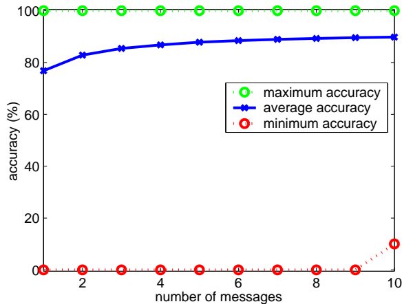
Figure 3: Plot showing the maximum, minimum and average accuracy of the prediction calculated using different numbers of messages, with r = 0.5 . This data is for all servers that send at least 10 messages. The best case has all predictions correct, the worst 1 correct out of 10. The average goes quickly to near 90%. This result highlights that accuracy improves with history (from 77% with one message to 90% with 10), and also that not much history ( < 10 messages) is needed to accurately predict message type.
