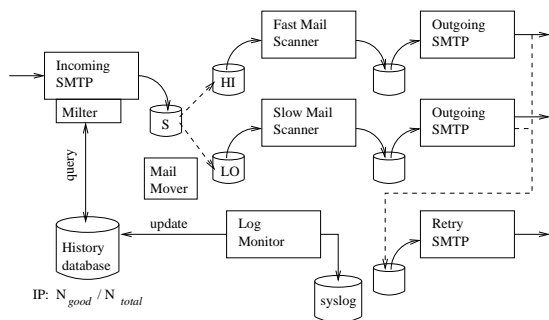
Figure 10: Schematic of implementation on sendmail. Mail is interrupted using the milter interface, and the milter queries the history database to determine for each connection whether to tempfail, or how to mark the message. Mail is placed in the spool S as usual, and moved into the appropriate queue by the MailMover process. The copied MailScanner then processes the two queues. Information about the message type is fed back from log files via the LogMonitor process.
