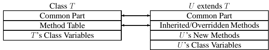
Figure 4: Class/Subclass Structures
