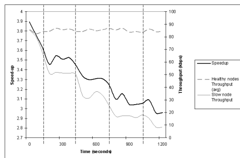
Figure 5: Agility of COMBINE with progressive reduction in WWAN speed of one of the collaborators
